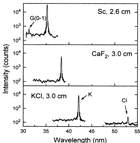
FIG. 2. Spectra for scandium, \text{CaF}_2 , and KCl with lasing on the J=0-1 , 3p\text{-}3s transitions. The weak G(0-1) line in scandium is indicated by an arrow, and the other lines are E(0-1) transitions. The total drive energy was 450 \pm 20 J with a 15% prepulse.
