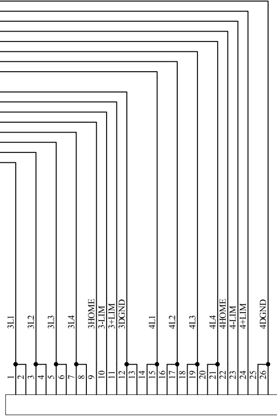
J2/4 CHANNELS 3&4 OR 7&8 26 PIN IDC
