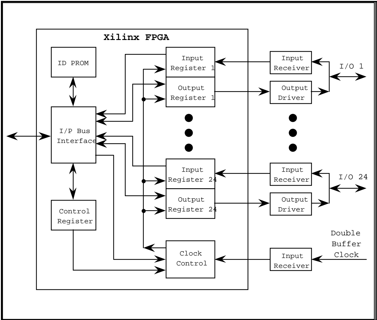
Figure 1 IP-UD Block Diagram
