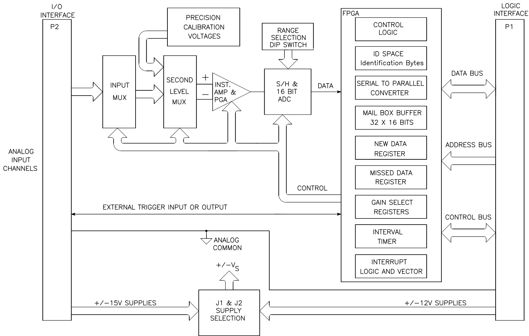
IP330 BLOCK DIAGRAM
