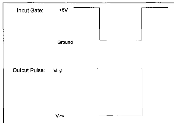
Generating a Negative Pulse With The PVX-4140
